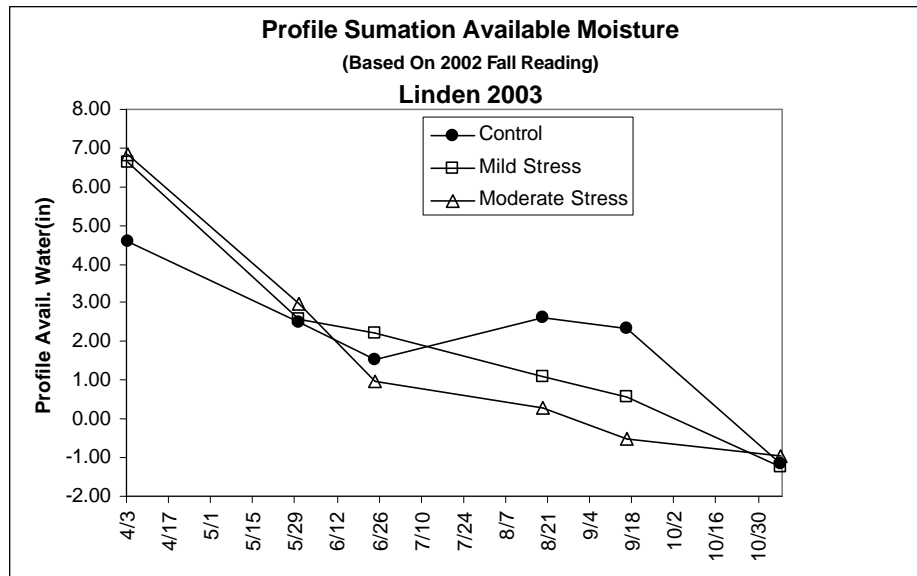
Figure 3. Average profile available moisture, as measured with a neutron probe, for Chandler walnuts at the San Joaquin County Site, 2003.
