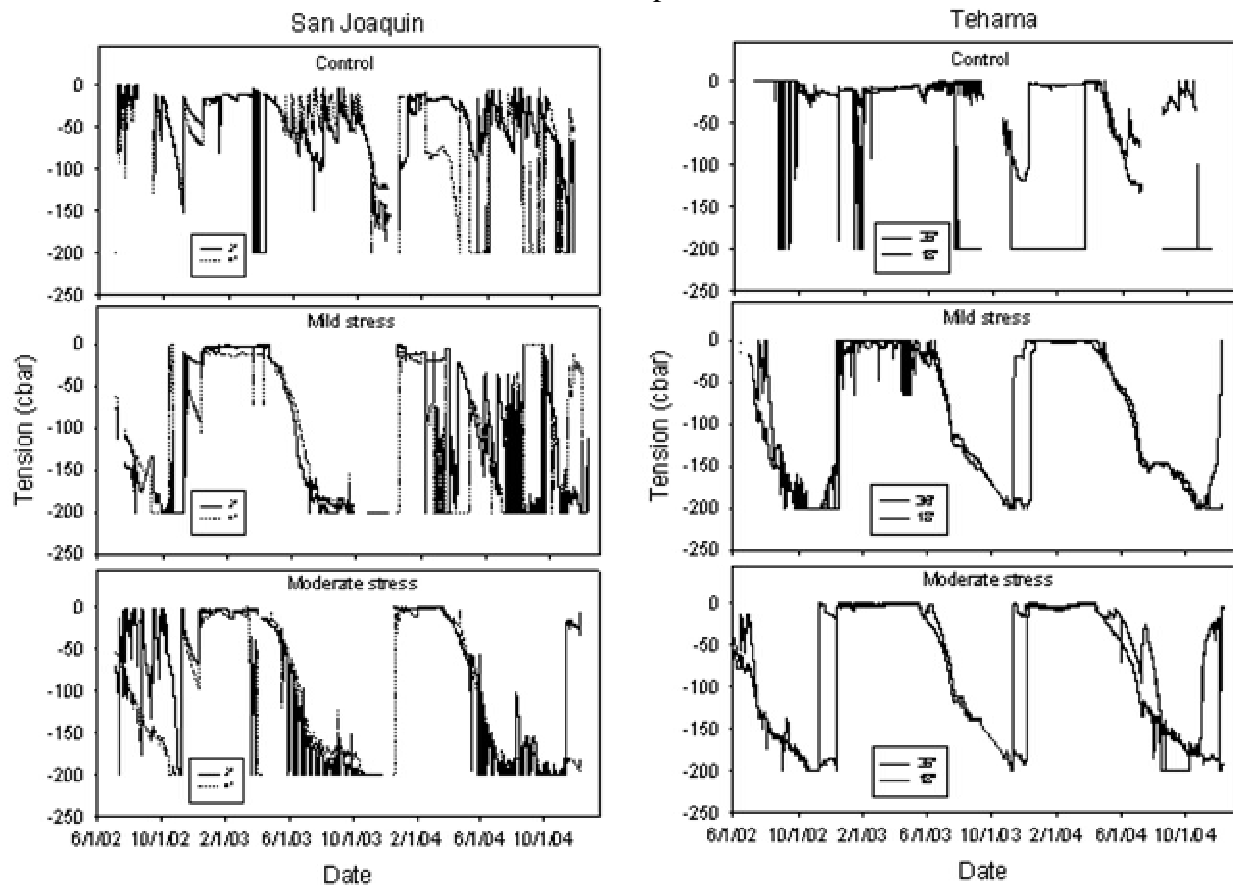
Figure 1. Soil moisture for the 2003 and 2004 season at the Tehama and San Joaquin County sites as measured with Watermark soil moisture sensors at two and four foot depths through season on control, mild stress and moderate stress plots.
