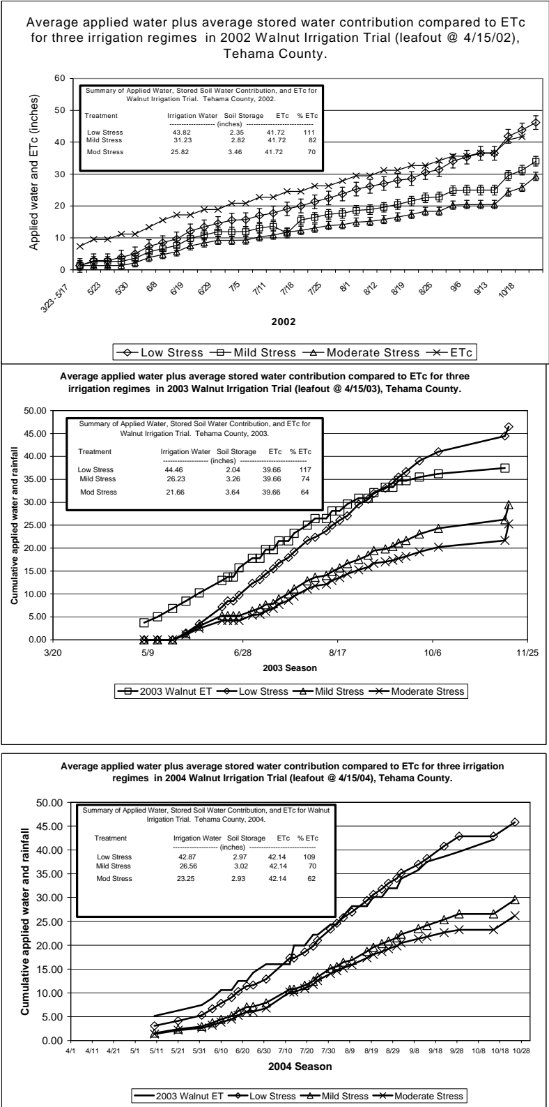
Figure 2. Average applied plus stored water and walnut evapotranspiration (ET) over 2002, 2003 and 2004 seasons for Tehama County site.
