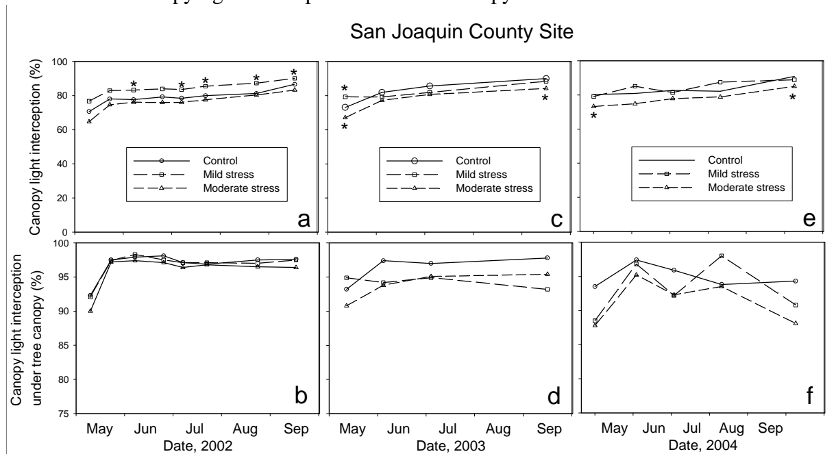
Figure 7. Canopy light interception for the 2002, 2003 and 2004 seasons at the San Joaquin County site as measured underneath (a,c,e) entire orchard and (b,d,f) underneath tree canopy only. Asterisk indicates significant difference from control. There were no significant treatment differences in canopy light interception under tree canopy.
